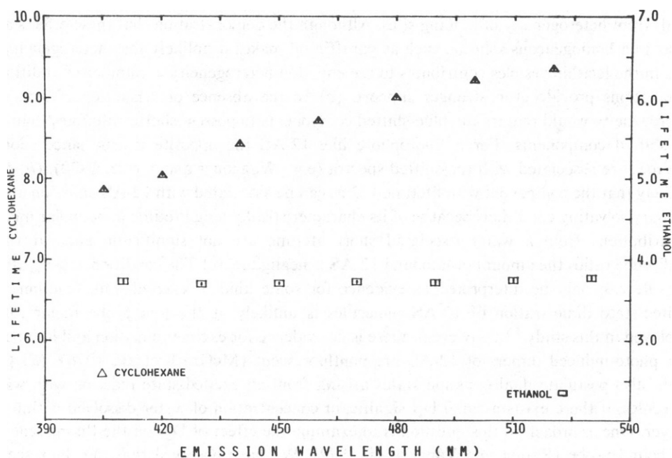
FIGURE 4 Modulation lifetimes (ns) (30 MHz) of 12-AS as a function of emission wavelength (nm) in ethanol ( \square ) and cyclohexane ( \Delta ). Samples were flushed with argon before measurement; temperature = 20°C.
