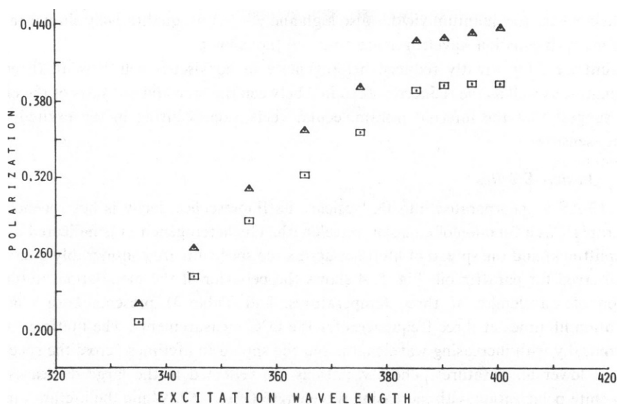
FIGURE 3 Polarization of 12-AS across its last absorption band. Sample contained 10 \mu M 12-AS in glycerol at 10°C. Excitation bandpass was 4 nm, emission bandpass (at 420 [ \Delta ] or 480 nm [ \square ]) was 8 nm. For purposes of demonstrating the mixed polarization across the absorption band, glycerol was chosen because the high polarization of 12-AS in this solvent maximized the changes in p value. The excitation wavelength is expressed in nanometers.
